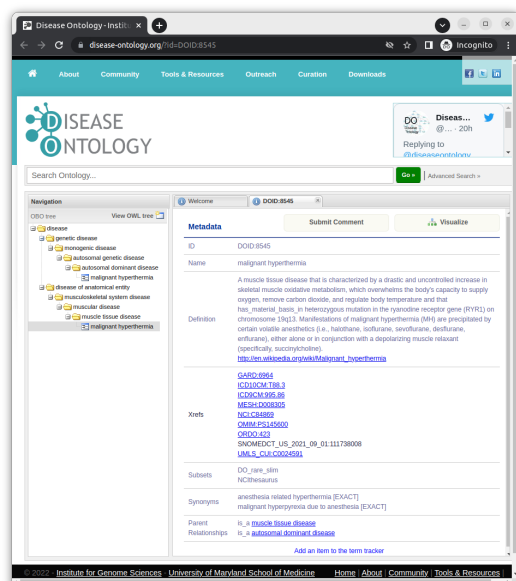
Fig. 3.10 Ontobee-Disease ontology entry for the class malignant hyperthermia
