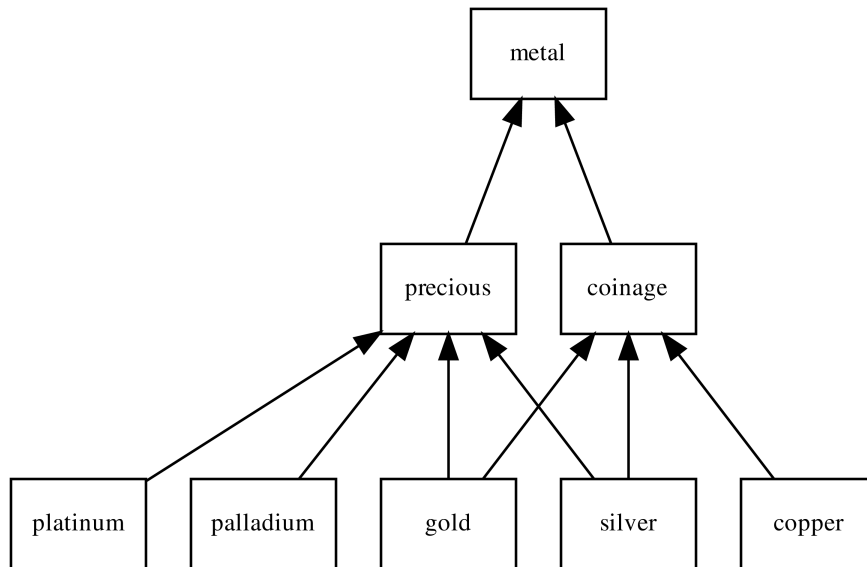
Fig. 2.1 A DAG representing a classification of metals with multiple inheritance, since gold and silver are considered both precious and coinage metals (All the links represent is-a relations)
